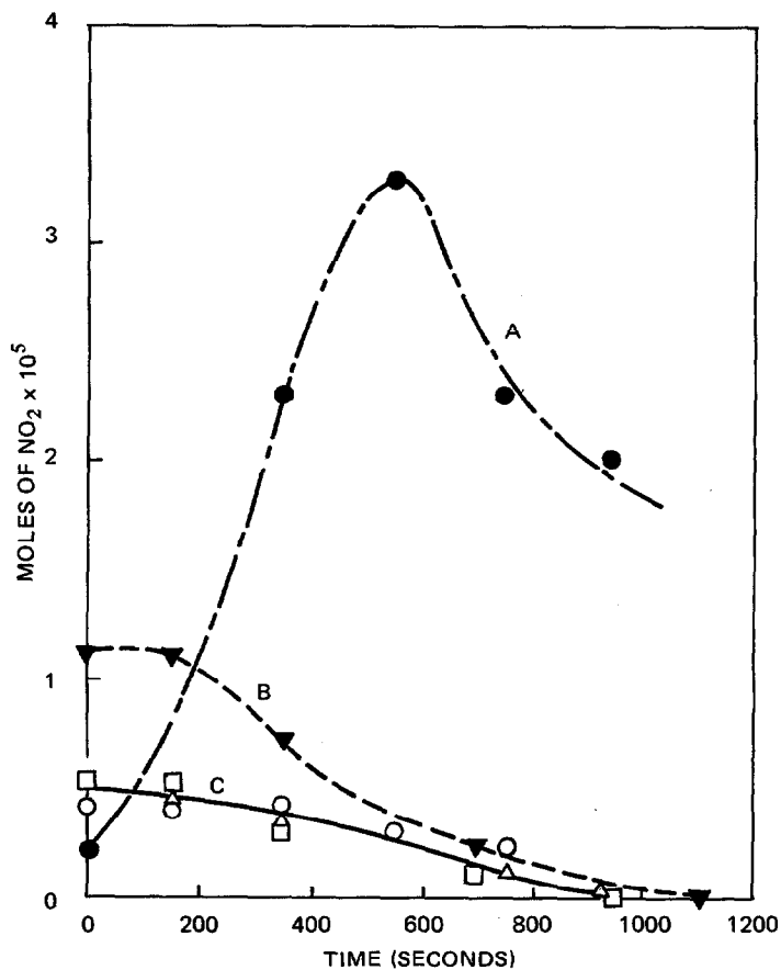
Fig 11 Concentration-time profiles of NO_2 for various initial weights of RDX and reactor volumes. Initial weights and volumes: A, 300ml, 40mg; B, 100ml, 40mg; C, 26ml, 12.5mg (o), 26mg ( \Delta ), 41.0mg ( \square )
